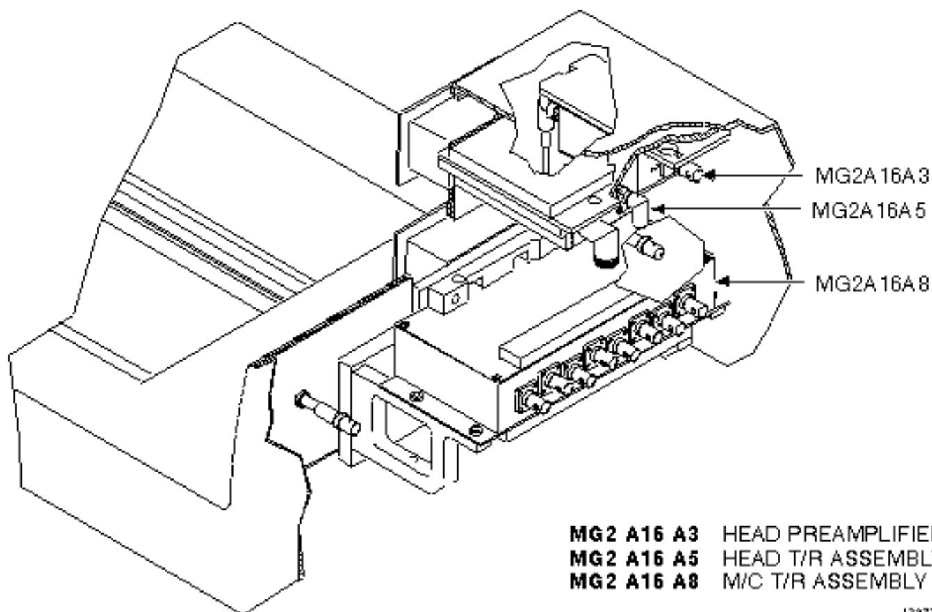
EXAM ROOM COMPONENT LOCATIONS (QUAD II HEAD COIL WITH MULTICOIL OPTION)
